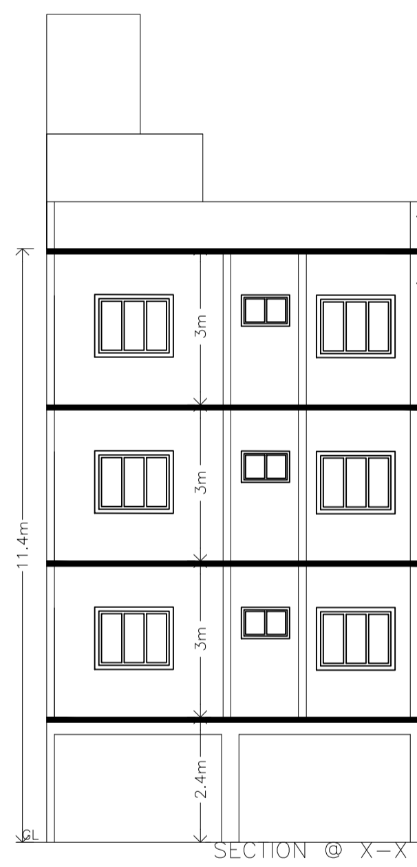
SECTION @ X-X
